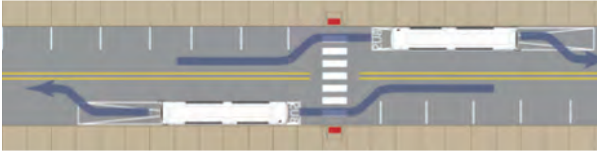
Figure 37a Placement of pedestrian crossing behind bus stops (Southeastern Pennsylvania Transport Authority 2012)
